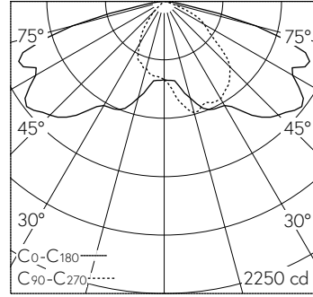
LED 4000 K 52.2 W 7376 lm-h H = 6 m / CIE Flux 38 75 96 100 100 / A30 nach DIN ...
