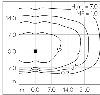
LED 4000 K 52.2 W 7376 lm-h H = 7 m / CIE Flux 38 75 96 100 100 / A30 nach DIN ...
