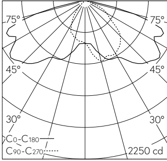
LED 4000 K 52.2 W 7376 lm-h H = 5 m / CIE Flux 38 75 96 100 100 / A30 nach DIN ...
