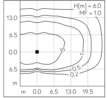
LED 4000 K 52.2 W 7376 lm-h H = 6 m / CIE Flux 38 75 96 100 100 / A30 nach DIN ...
