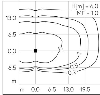
LED 3000 K 52.2 W 7170 lm-h H = 6 m / CIE Flux 38 75 96 100 100 / A30 nach DIN ...
