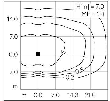
LED 3000 K 52.2 W 7170 lm-h H = 7 m / CIE Flux 38 75 96 100 100 / A30 nach DIN ...
