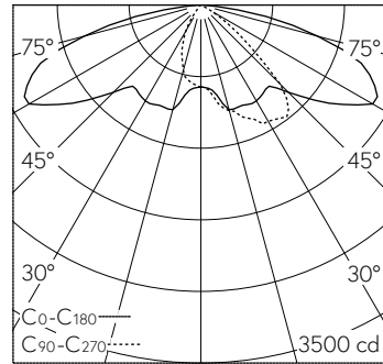
LED 4000 K 34.5 W 4683 lm-h H = 8 m / CIE Flux 34 68 94 100 100 / A20 nach DIN ...
