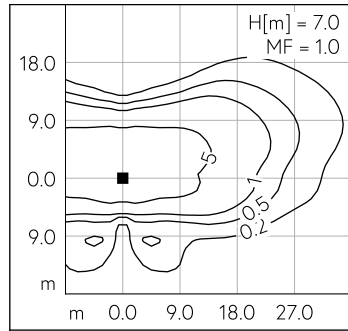
LED 4000 K 34.5 W 4683 lm-h H = 7 m / CIE Flux 34 68 94 100 100 / A20 nach DIN ...
