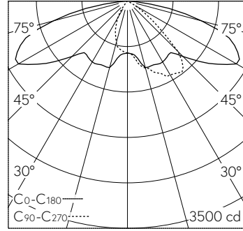
LED 4000 K 34.5 W 4683 lm-h H = 5 m / CIE Flux 34 68 94 100 100 / A20 nach DIN ...
