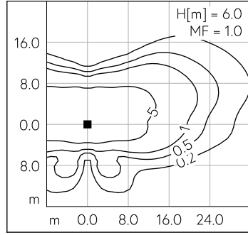
LED 4000 K 34.5 W 4683 lm-h H = 6 m / CIE Flux 34 68 94 100 100 / A20 nach DIN ...
