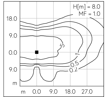
LED 4000 K 34.5 W 4683 lm-h H = 8 m / CIE Flux 34 68 94 100 100 / A20 nach DIN ...
