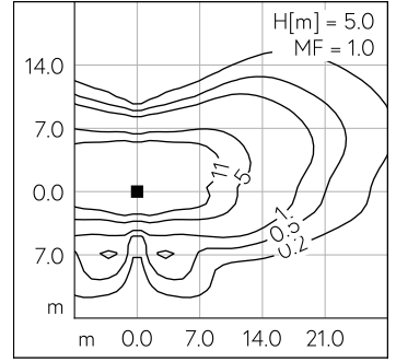
LED 4000 K 34.5 W 4683 lm-h H = 5 m / CIE Flux 34 68 94 100 100 / A20 nach DIN ...
