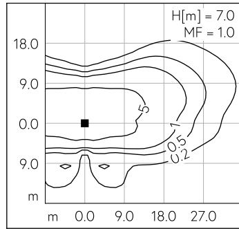
LED 3000 K 34.5 W 4554 lm-h H = 7 m / CIE Flux 34 68 94 100 100 / A20 nach DIN ...
