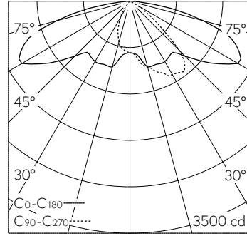
LED 3000 K 34.5 W 4554 lm-h H = 5 m / CIE Flux 34 68 94 100 100 / A20 nach DIN ...
