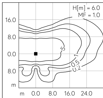
LED 4000 K 67 W 9366 lm-h H = 6 m / CIE Flux 34 68 94 100 100 / A20 nach DIN 5...
