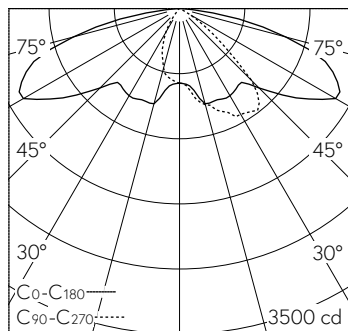
LED 4000 K 67 W 9366 lm-h H = 8 m / CIE Flux 34 68 94 100 100 / A20 nach DIN 5...
