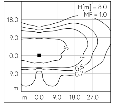
LED 3000 K 67 W 9108 lm-h H = 8 m / CIE Flux 34 68 94 100 100 / A20 nach DIN 5...
