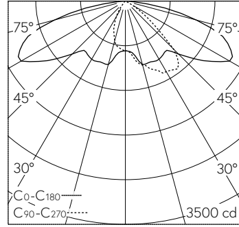
LED 3000 K 67 W 9108 lm-h H = 5 m / CIE Flux 34 68 94 100 100 / A20 nach DIN 5...
