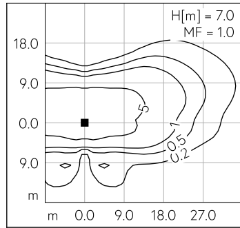
LED 3000 K 67 W 9108 lm-h H = 7 m / CIE Flux 34 68 94 100 100 / A20 nach DIN 5...
