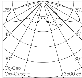
LED 3000 K 67 W 9108 lm-h H = 8 m / CIE Flux 34 68 94 100 100 / A20 nach DIN 5...
