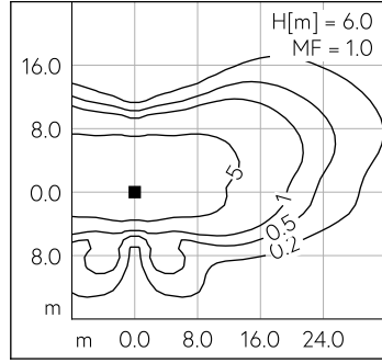
LED 3000 K 67 W 9108 lm-h H = 6 m / CIE Flux 34 68 94 100 100 / A20 nach DIN 5...
