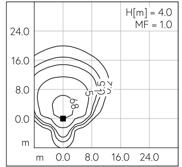
LED 3000 K 58.5 W 7059 lm-h H = 4 m / CIE Flux 39 80 99 100 100 / A30 nach DIN...
