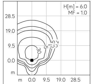
LED 3000 K 58.5 W 7059 lm-h H = 6 m / CIE Flux 39 80 99 100 100 / A30 nach DIN...
