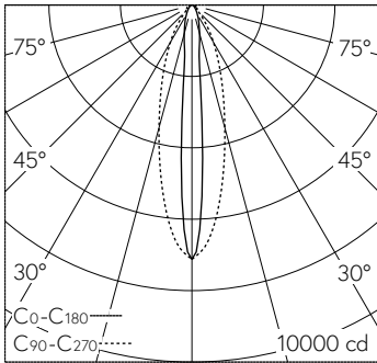
LED 4000 K 20.9 W 1511 lm-h 9.4°/30° 71120M / CIE Flux 84 95 99 100 100 / A70 na...
