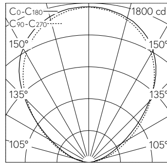
LED 3000 K 36.1 W 4168 lm-h / CIE Flux 0 0 0 100 / E83 nach DIN 5040
