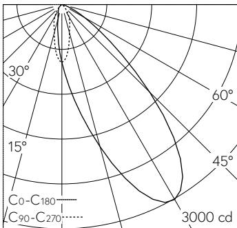
LED 3000 K 13.5 W 1190 lm-h 30° B10014 / CIE Flux 74 97 100 100 100 / A70 nach ...
