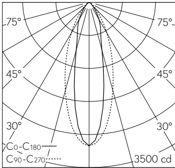
LED 3000 K 13.5 W 1338 lm-h 24°/38° B10014 / CIE Flux 89 99 100 100 100 / A80 n...
