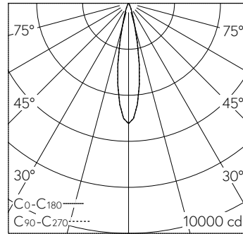
LED 3000 K 13.5 W 834 lm-h 20° B71215 / CIE Flux 98 100 100 100 100 / A80 nach ...
