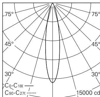
LED 4000 K 20 W 2264 lm-h 20° / CIE Flux 98 100 100 100 100 / A80 selon DIN 5040
