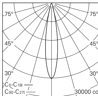
LED 3000 K 36 W 2825 lm-h 18.0° / CIE Flux 99 100 100 100 100 / A80 selon DIN 5...
