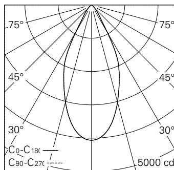
LED 3000 K 31 W 2499 lm-h 48° / CIE Flux 94 99 100 100 100 / A80 selon DIN 5040
