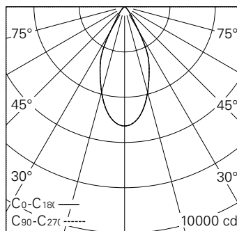
LED 4000 K 27 W 3242 lm-h 48° / CIE Flux 94 99 100 100 100 / A80 selon DIN 5040
