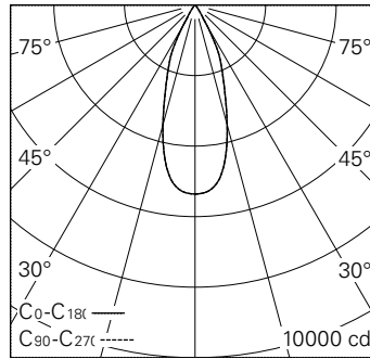
LED 3000 K 27 W 2390 lm-h 38° / CIE Flux 98 100 100 100 100 / A80 selon DIN 5040
