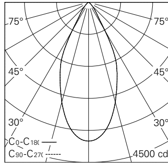
LED 4000 K 20 W 2399 lm-h 48° / CIE Flux 94 99 100 100 100 / A80 selon DIN 5040
