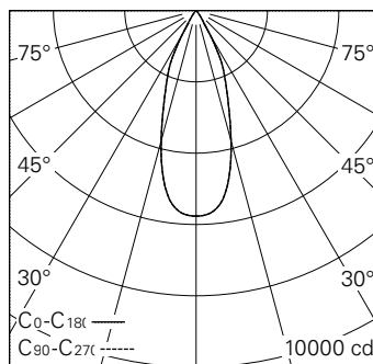
LED 4000 K 20 W 2572 lm-h 38° / CIE Flux 98 100 100 100 100 / A80 selon DIN 5040
