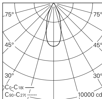
LED 2700 K 20 W 1995 lm-h 38° / CIE Flux 98 100 100 100 100 / A80 selon DIN 5040
