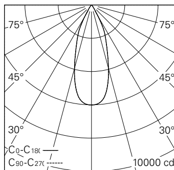
LED 3000 K 31 W 2680 lm-h 38° / CIE Flux 98 100 100 100 100 / A80 selon DIN 5040
