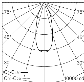
LED 3000 K 27 W 2760 lm-h 38° / CIE Flux 98 100 100 100 100 / A80 selon DIN 5040
