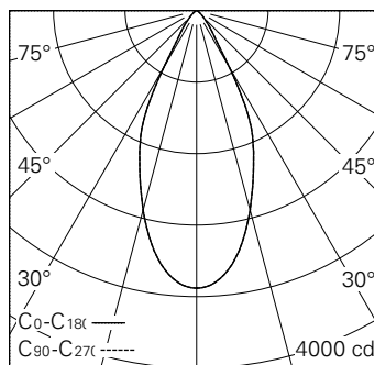
LED 3000 K 20 W 1910 lm-h 48° / CIE Flux 94 99 100 100 100 / A80 selon DIN 5040
