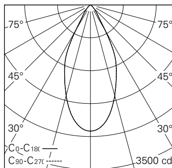
LED 3000 K 20 W 1651 lm-h 48° / CIE Flux 94 99 100 100 100 / A80 selon DIN 5040
