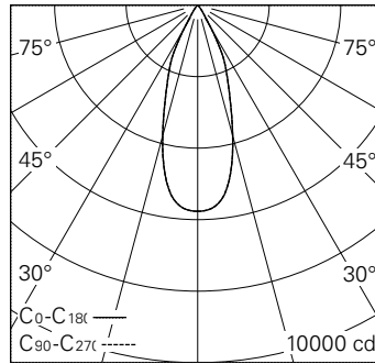
LED 4000 K 20 W 2572 lm-h 38° / CIE Flux 98 100 100 100 100 / A80 selon DIN 5040
