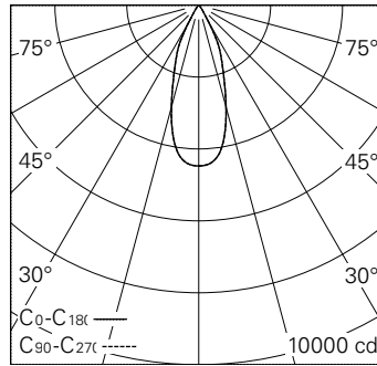
LED 2700 K 20 W 1995 lm-h 38° / CIE Flux 98 100 100 100 100 / A80 selon DIN 5040
