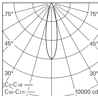
LED 3000 K 14 W 1349 lm-h 22° / CIE Flux 98 100 100 100 100 / A80 selon DIN 5040
