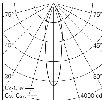
LED 3000 K 11 W 826 lm-h 24° / CIE Flux 100 100 100 100 100 / A80 selon DIN 5040
