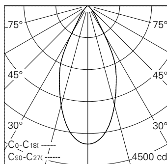
LED 4000 K 20 W 2399 lm-h 48° / CIE Flux 94 99 100 100 100 / A80 selon DIN 5040
