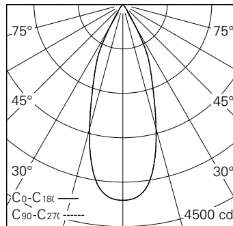
LED 3000 K 20 W 1770 lm-h 38° / CIE Flux 98 100 100 100 100 / A80 selon DIN 5040
