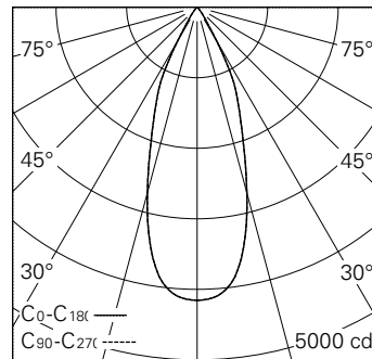
LED 4000 K 14 W 1853 lm-h 38° / CIE Flux 98 100 100 100 100 / A80 selon DIN 5040
