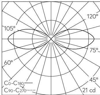
LED 3000 K 19,5 W 618 lm-h 132° / CIE Flux 1 13 46 49 100 / C11 selon DIN 5040
