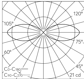
LED 3000 K 3,0 W 89 lm-h 134° / CIE Flux 1 14 47 51 100 / C11 selon DIN 5040
