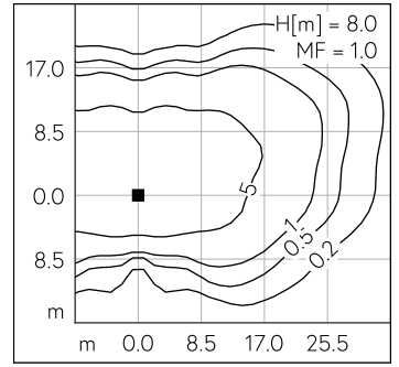
LED 4000 K 53 W 7770 lm-h H = 8 m / CIE Flux 33 72 98 100 100 / A20 selon DIN 5...
