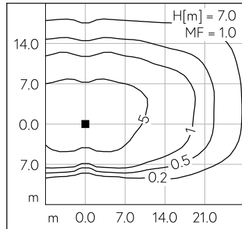
LED 4000 K 52.2 W 7376 lm-h H = 7 m / CIE Flux 38 75 96 100 100 / A30 selon DIN ...
