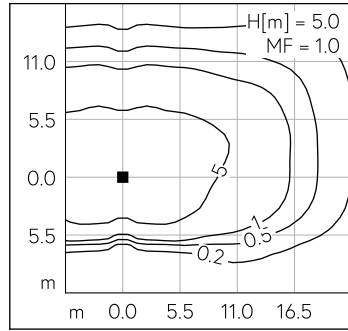
LED 4000 K 52.2 W 7376 lm-h H = 5 m / CIE Flux 38 75 96 100 100 / A30 selon DIN...
