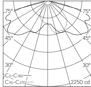
LED 4000 K 52.2 W 7376 lm-h H = 6 m / CIE Flux 38 75 96 100 100 / A30 selon DIN...
