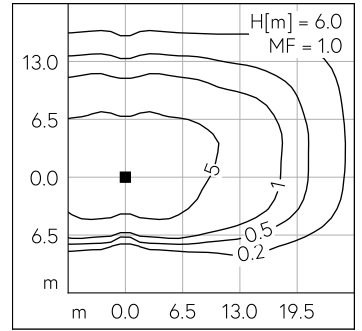
LED 4000 K 52.2 W 7376 lm-h H = 6 m / CIE Flux 38 75 96 100 100 / A30 selon DIN...
