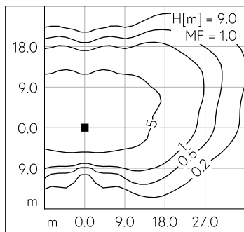
LED 4000 K 53 W 7770 lm-h H = 9 m / CIE Flux 33 71 97 100 100 / A20 selon DIN 5...
