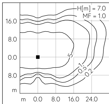
LED 4000 K 53 W 7770 lm-h H = 7 m / CIE Flux 33 71 97 100 100 / A20 selon DIN 5...
