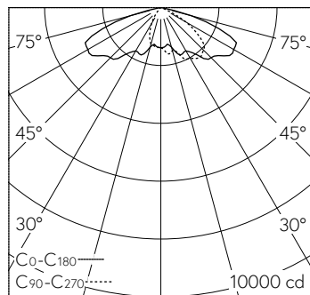
LED 4000 K 53 W 7770 lm-h H = 8 m / CIE Flux 33 71 97 100 100 / A20 selon DIN 5...
