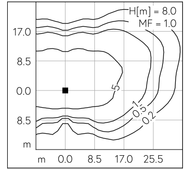
LED 3000 K 53 W 7553 lm-h H = 8 m / CIE Flux 33 71 97 100 100 / A20 selon DIN 5...
