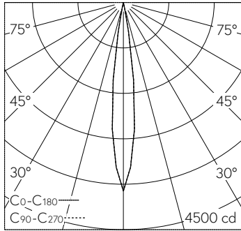
LED O K 39 W 281 lm-h 13.4°_Spot / CIE Flux 100 100 100 100 100 / A80 selon DIN ...
