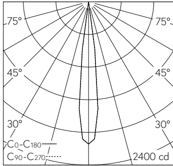
LED O K 18 W 196 lm-h 13.0°_Spot / CIE Flux 100 100 100 100 100 / A80 selon DIN ...
