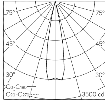
LED 4000 K 24 W 310 lm-h 20°_Flood / CIE Flux 100 100 100 100 100 / A80 selon D...
