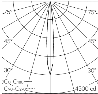
LED 4000 K 24 W 310 lm-h 10.8°_Spot / CIE Flux 100 100 100 100 100 / A80 selon ...
