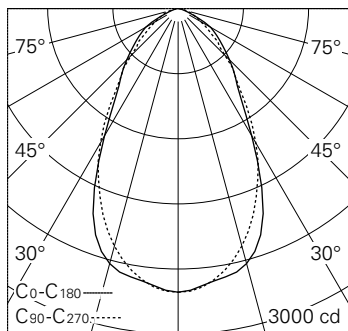
LED 3000 K 40 W 3485 lm-h 62°/64° B71113 / CIE Flux 72 93 99 100 100 / A60 selon DIN 5040
