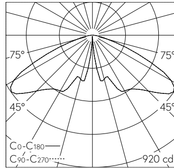
LED 4000 K 22.2 W 1498 lm-h / CIE Flux 30 73 96 99 100 / A20 selon DIN 5040
