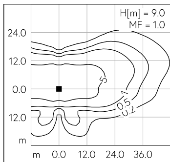
LED 3000 K 69 W 9163 lm-h H = 9 m / CIE Flux 34 66 93 100 100 / A20 selon DIN 5...
