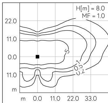
LED 3000 K 69 W 9163 lm-h H = 8 m / CIE Flux 34 66 93 100 100 / A20 selon DIN 5...
