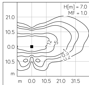
LED 3000 K 69 W 9163 lm-h H = 7 m / CIE Flux 34 66 93 100 100 / A20 selon DIN 5...
