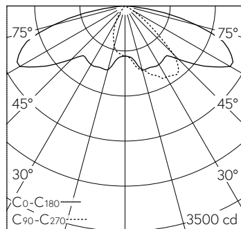
LED 3000 K 34.5 W 4554 lm-h H = 8 m / CIE Flux 34 68 94 100 100 / A20 selon DIN...
