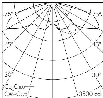
LED 3000 K 34.5 W 4554 lm-h H = 7 m / CIE Flux 34 68 94 100 100 / A20 selon DIN...
