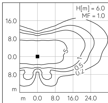
LED 3000 K 34.5 W 4554 lm-h H = 6 m / CIE Flux 34 68 94 100 100 / A20 selon DIN...
