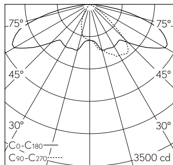
LED 3000 K 34.5 W 4554 lm-h H = 5 m / CIE Flux 34 68 94 100 100 / A20 selon DIN...
