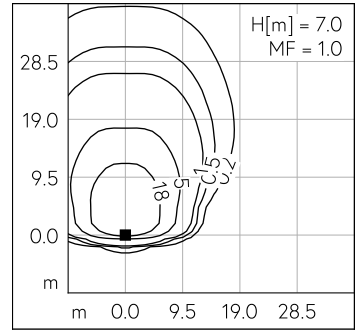
LED 3000 K 51 W 7692 lm-h H = 7 m / CIE Flux 37 74 96 100 100 / A30 selon DIN 5...
