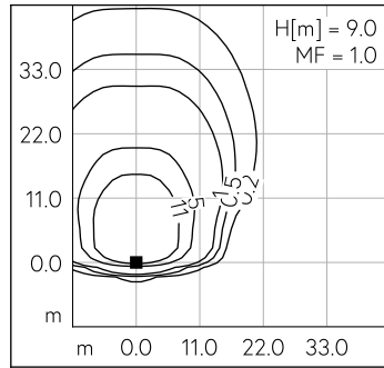
LED 3000 K 51 W 7692 lm-h H = 9 m / CIE Flux 37 74 96 100 100 / A30 selon DIN 5...
