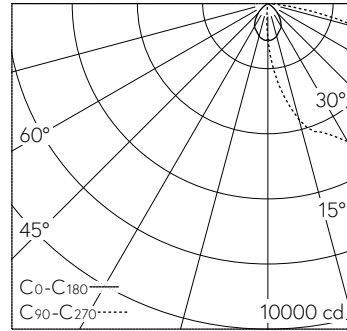
LED 3000 K 51 W 7692 lm-h H = 7 m / CIE Flux 37 74 96 100 100 / A30 selon DIN 5...
