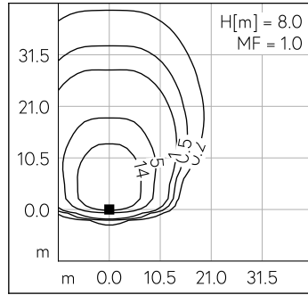
LED 3000 K 51 W 7692 lm-h H = 8 m / CIE Flux 37 74 96 100 100 / A30 selon DIN 5...
