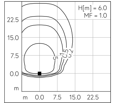
LED 4000 K 18.8 W 2649 lm-h H = 6 m / CIE Flux 34 72 95 100 100 / A30 selon DIN ...
