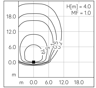
LED 4000 K 18.8 W 2649 lm-h H = 4 m / CIE Flux 34 72 95 100 100 / A30 selon DIN ...
