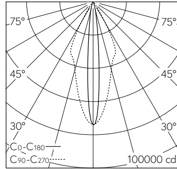
LED 4000 K 312 W 14327 lm-h 71101M / CIE Flux 98 100 100 100 100 / A80 selon DI...
