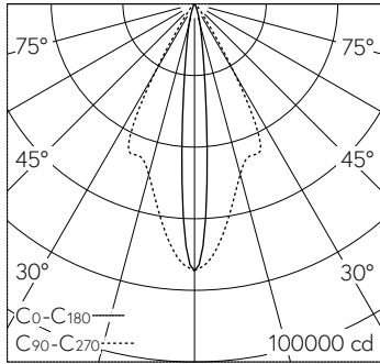
LED 4000 K 312 W 15077 lm-h 11.4°/52° / CIE Flux 97 100 100 100 100 / A80 selon ...
