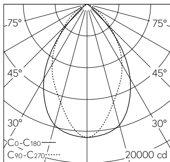
LED 4000 K 190 W 20949 lm-h 70°/62° / CIE Flux 77 97 100 100 100 / A70 selon DI...
