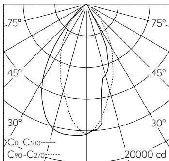
LED 4000 K 190 W 13726 lm-h 71108M / CIE Flux 85 98 100 100 100 / A70 selon DI...
