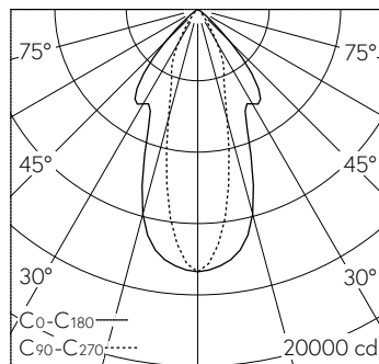
LED 4000 K 190 W 8206 lm-h 44°/28° 71107M / CIE Flux 89 99 100 100 100 / A80 s...
