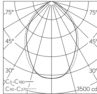
LED RGBW 0 K 59 W 4838 lm-h 82°/84° / CIE Flux 66 93 99 100 100 / A60 selon DL...
