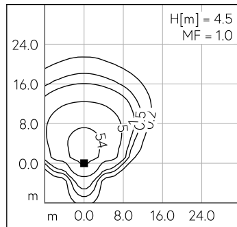
LED 4000 K 117 W 14320 lm-h H = 4.5 m / CIE Flux 39 80 99 100 100 / A30 selon DI...
