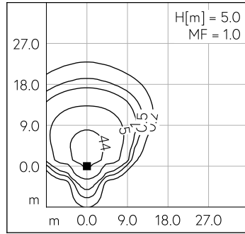
LED 4000 K 117 W 14320 lm-h H = 5 m / CIE Flux 39 80 99 100 100 / A30 selon DIN...
