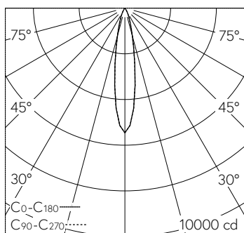
LED 3000 K 19 W 971 lm-h 18.8° 71119M / CIE Flux 98 100 100 100 100 / A80 selon ...
