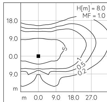
LED 3000 K 68 W 9290 lm-h H = 8 m / CIE Flux 35 69 94 100 100 / A30 selon DIN ...
