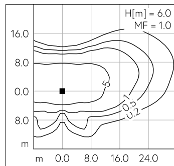
LED 3000 K 68 W 9290 lm-h H = 6 m / CIE Flux 35 69 94 100 100 / A30 selon DIN 5...
