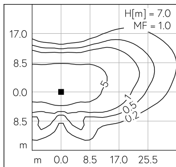
LED 3000 K 68 W 9290 lm-h H = 7 m / CIE Flux 35 69 94 100 100 / A30 selon DIN 5...
