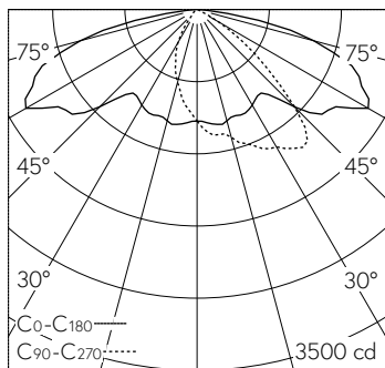
LED 3000 K 68 W 9290 lm-h H = 5 m / CIE Flux 35 69 94 100 100 / A30 selon DIN ...
