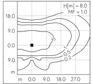
LED 3000 K 34 W 4645 lm-h H = 8 m / CIE Flux 35 69 94 100 100 / A30 selon DIN 5...
