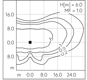
LED 3000 K 34 W 4645 lm-h H = 6 m / CIE Flux 35 69 94 100 100 / A30 selon DIN 5...
